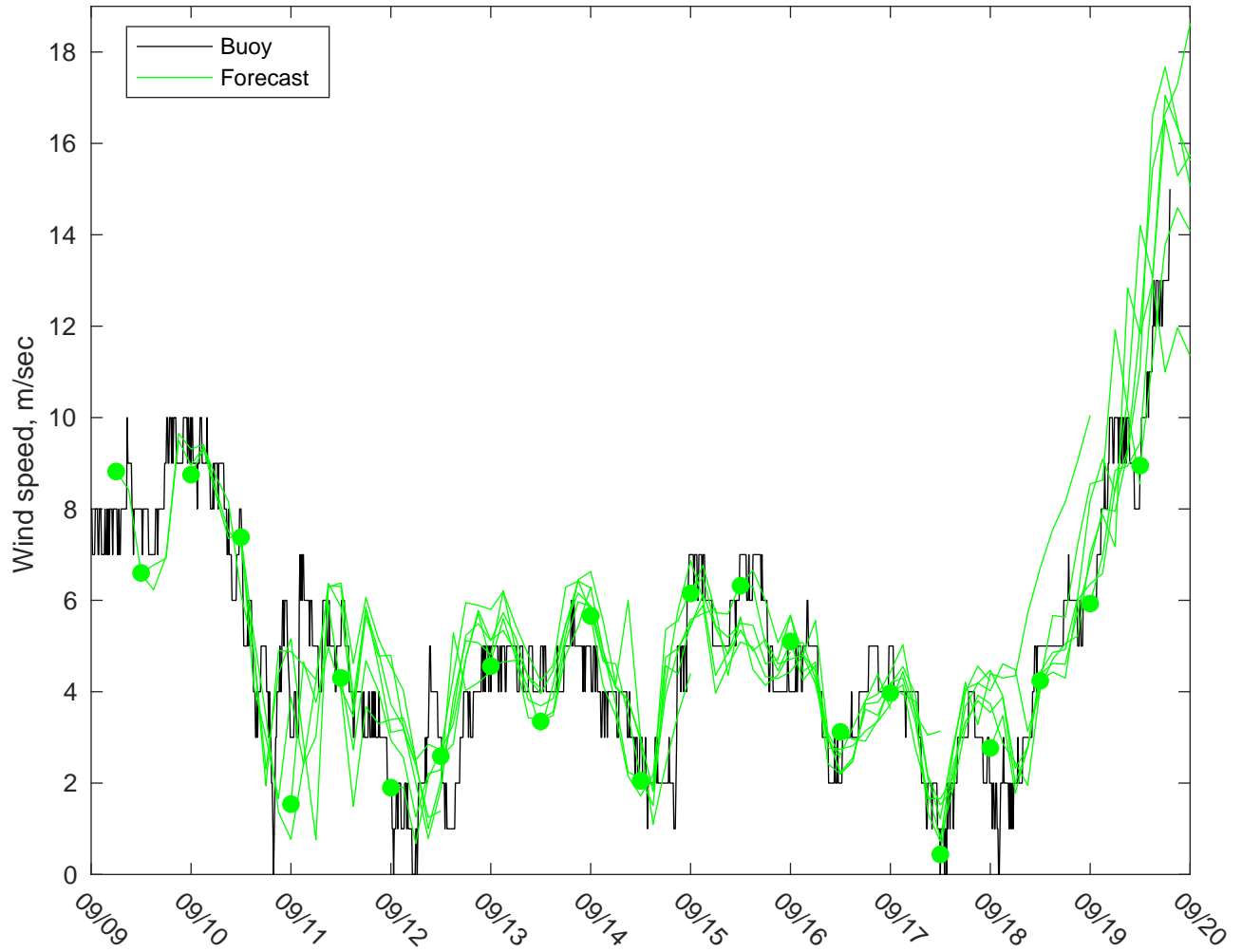
NDBC 44020 vs GFSWinds: 0 to 3 day forecast
