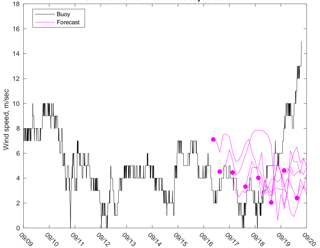
NDBC 44020 vs GFSWinds: 7 to 10 day forecast
