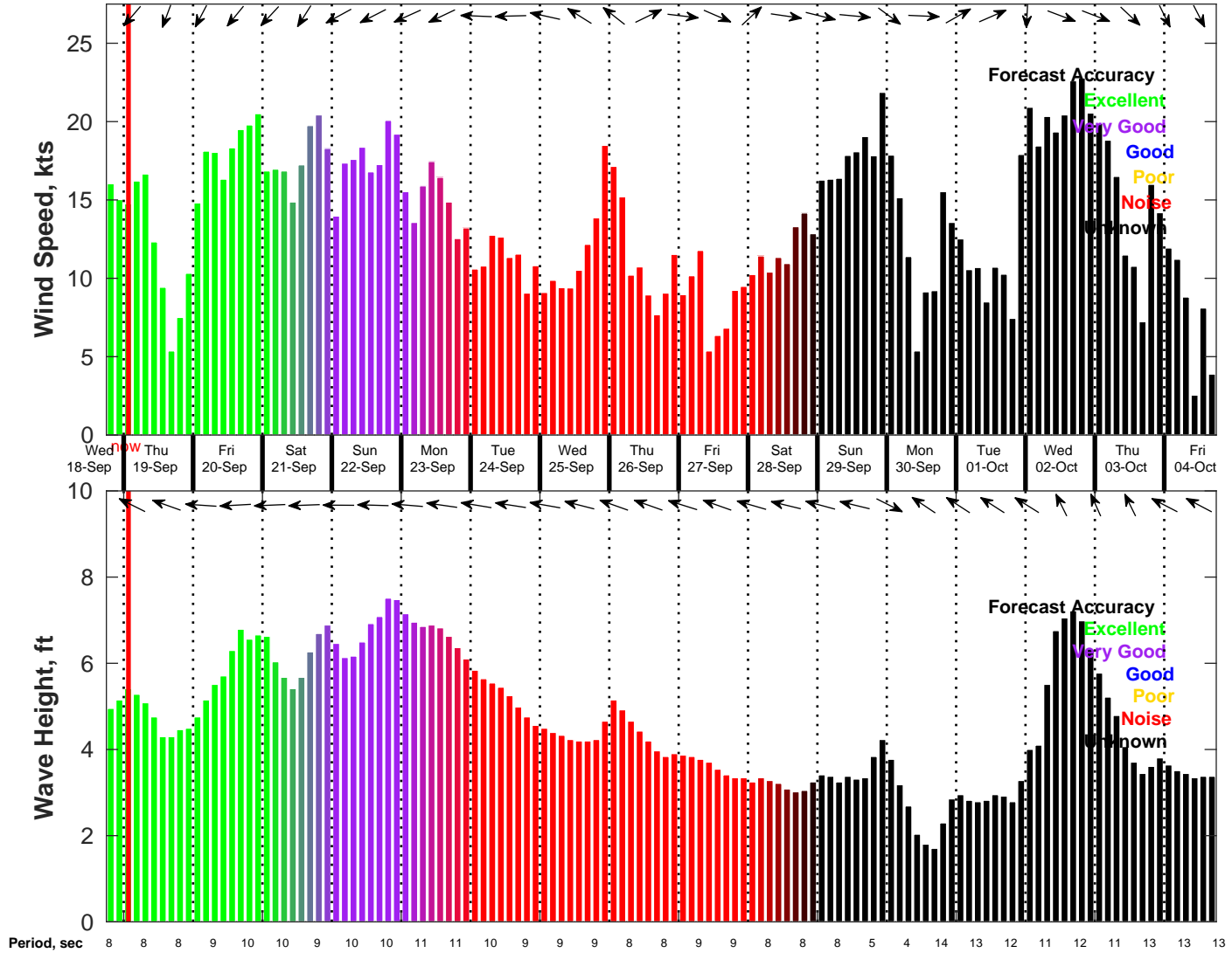
Wind & Wave Forecast for NDBC 44025 from 18-Sep-2024 18:00:00 to 04-Oct-2024 18:00:00
