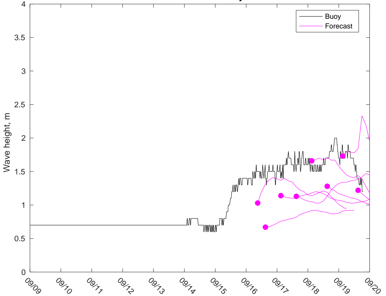
NDBC 44025 vs GFSWaves: 7 to 10 day forecast
