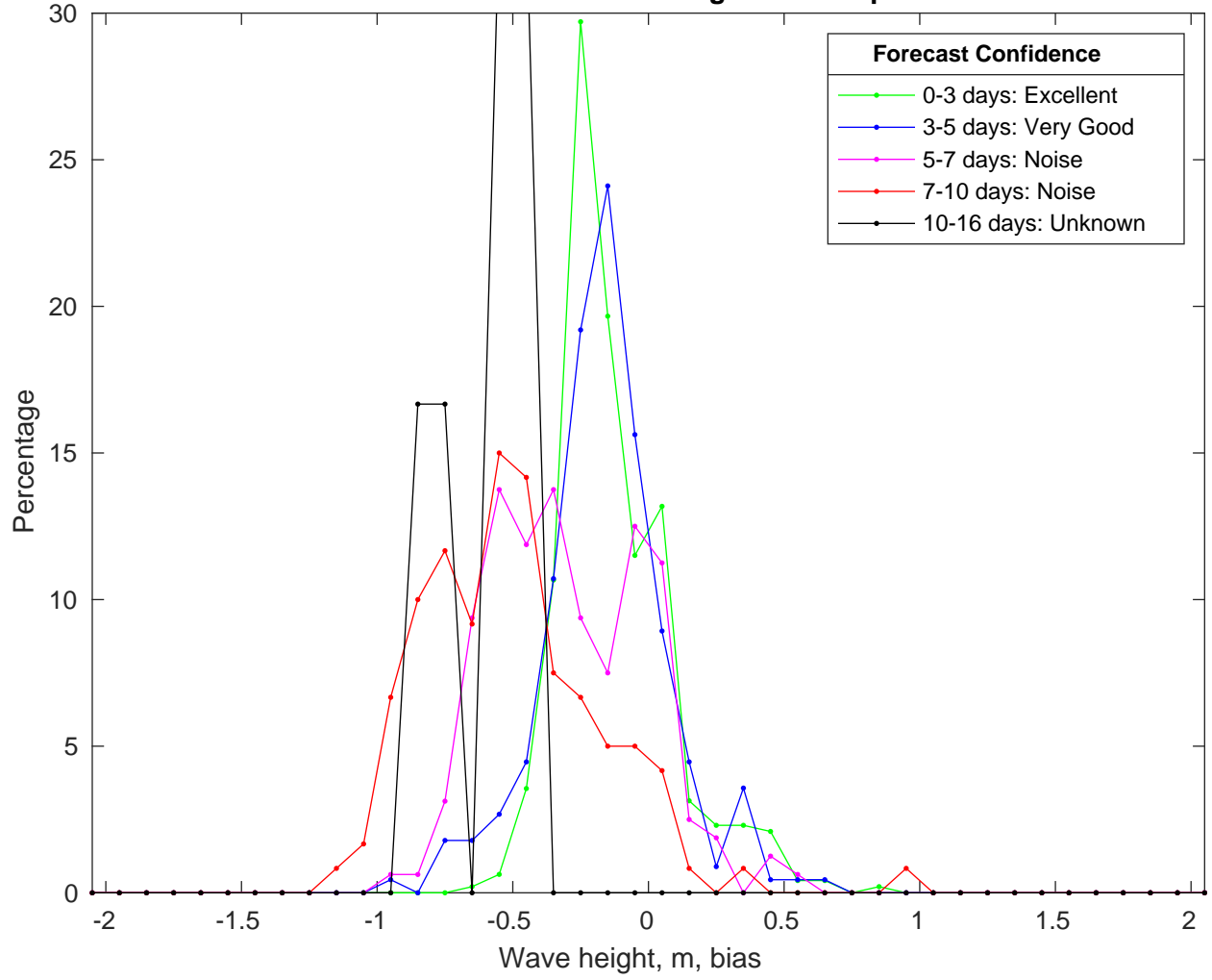
NDBC 44025 vs GFSWaves Bias Histogram: 19-Sep-2024
