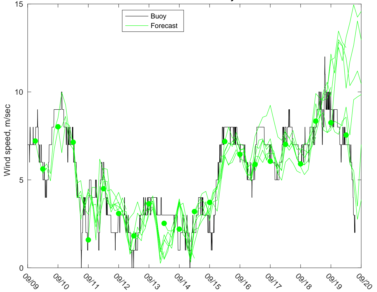
NDBC 44025 vs GFSWinds: 0 to 3 day forecast
