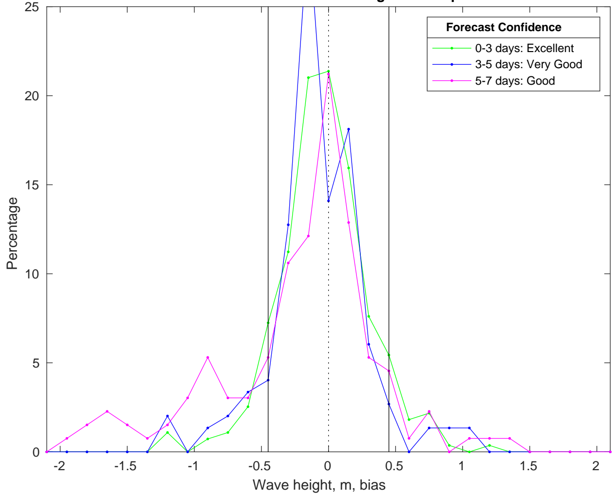
NDBC 46011 vs AUSWAV Waves Bias Histogram: 04-Apr-2025
