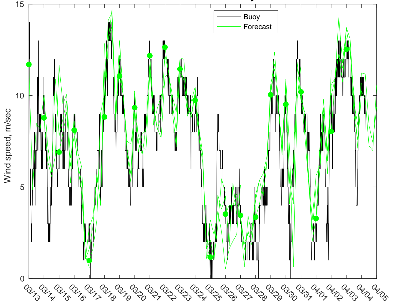
NDBC 46011 vs AUSWAV Winds: 0 to 3 day forecast
