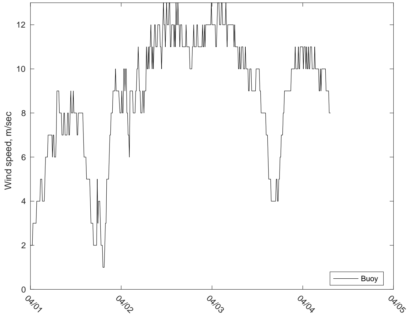
NDBC 46011 vs AUSWAV Winds: 10 to 16 day forecast
