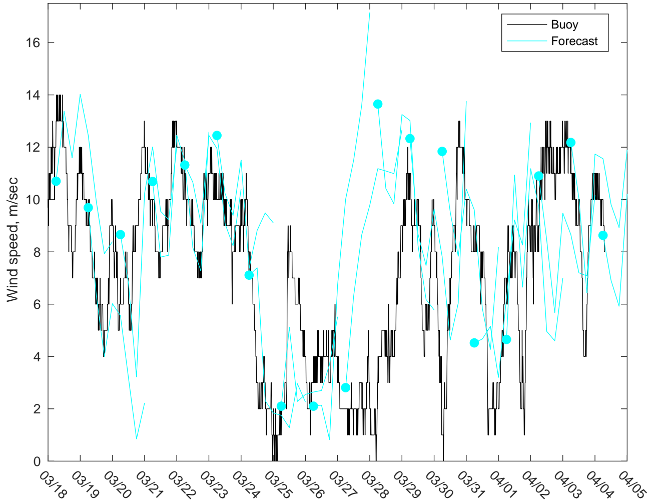
NDBC 46011 vs AUSWAV Winds: 5 to 7 day forecast
