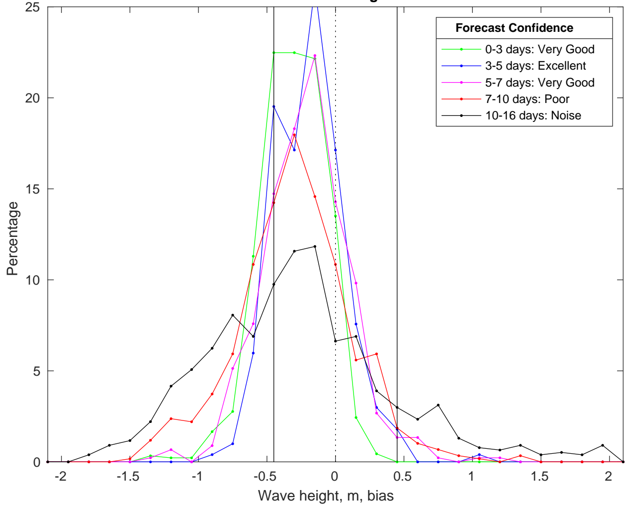
NDBC 46011 vs GFSWaves Bias Histogram: 18-Jan-2025
