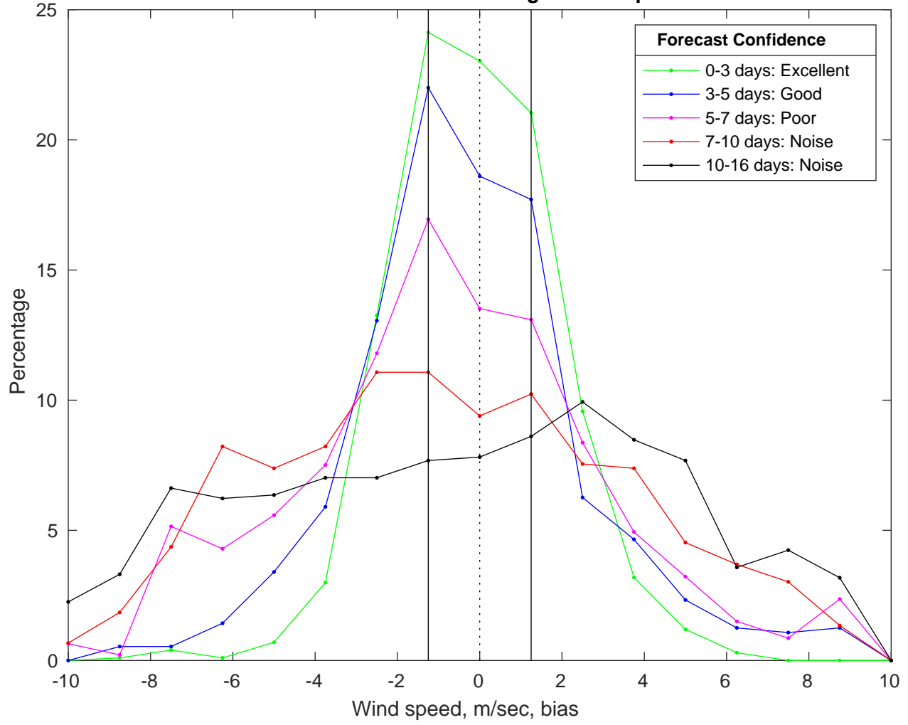
NDBC 46011 vs GFS Winds Bias Histogram: 04-Apr-2025
