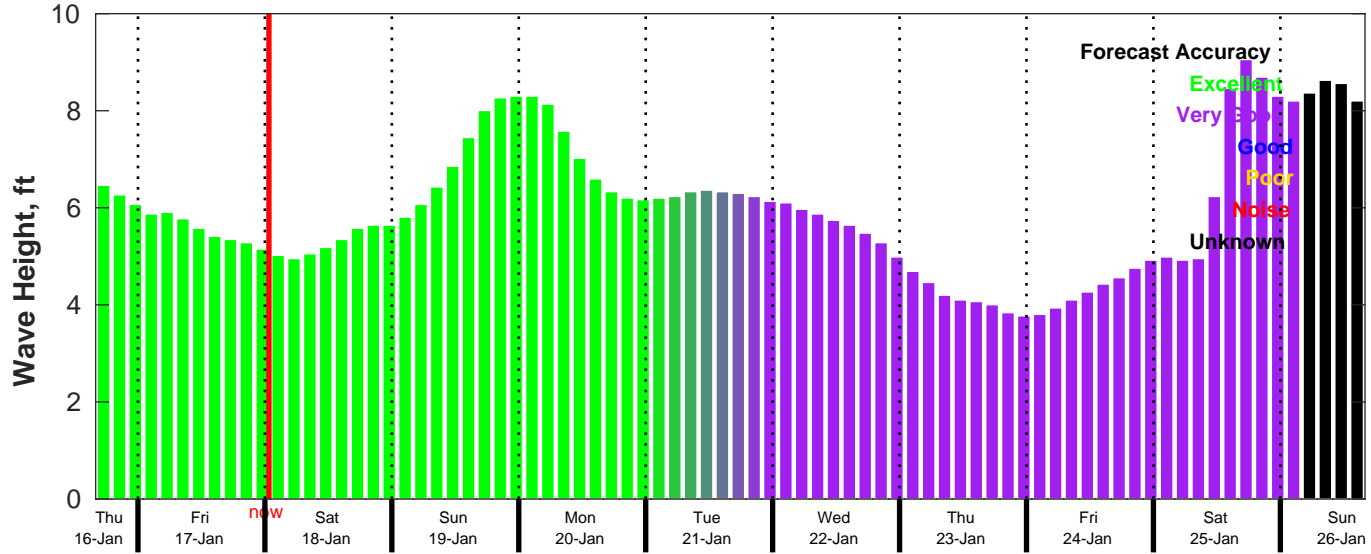
CMEMS Wave Forecast for NDBC 46011 from 16-Jan-2025 16:00:00 to 26-Jan-2025 16:00:00
