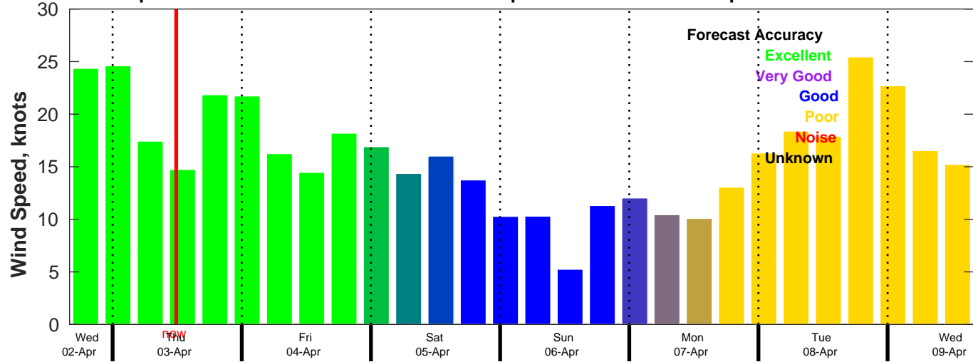
AUSWAV Wind Speed Forecast for NDBC 46011 from 02-Apr-2025 16:00:00 to 09-Apr-2025 16:00:00
