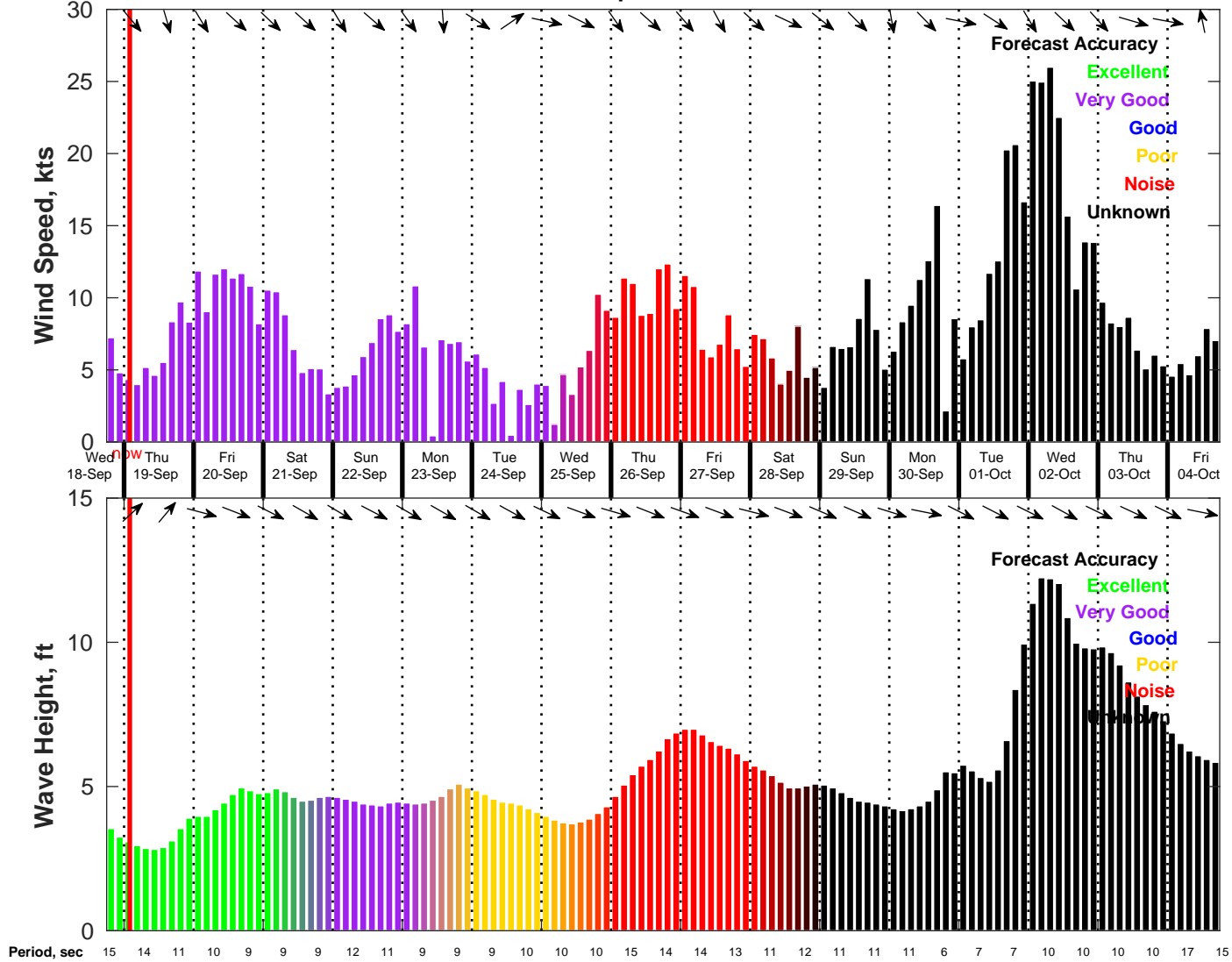
Wind & Wave Forecast for NDBC 46011 from 18-Sep-2024 18:00:00 to 04-Oct-2024 18:00:00
