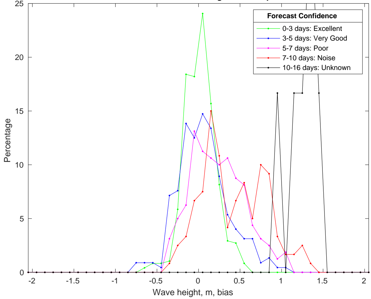
NDBC 46011 vs GFSWaves Bias Histogram: 19-Sep-2024
