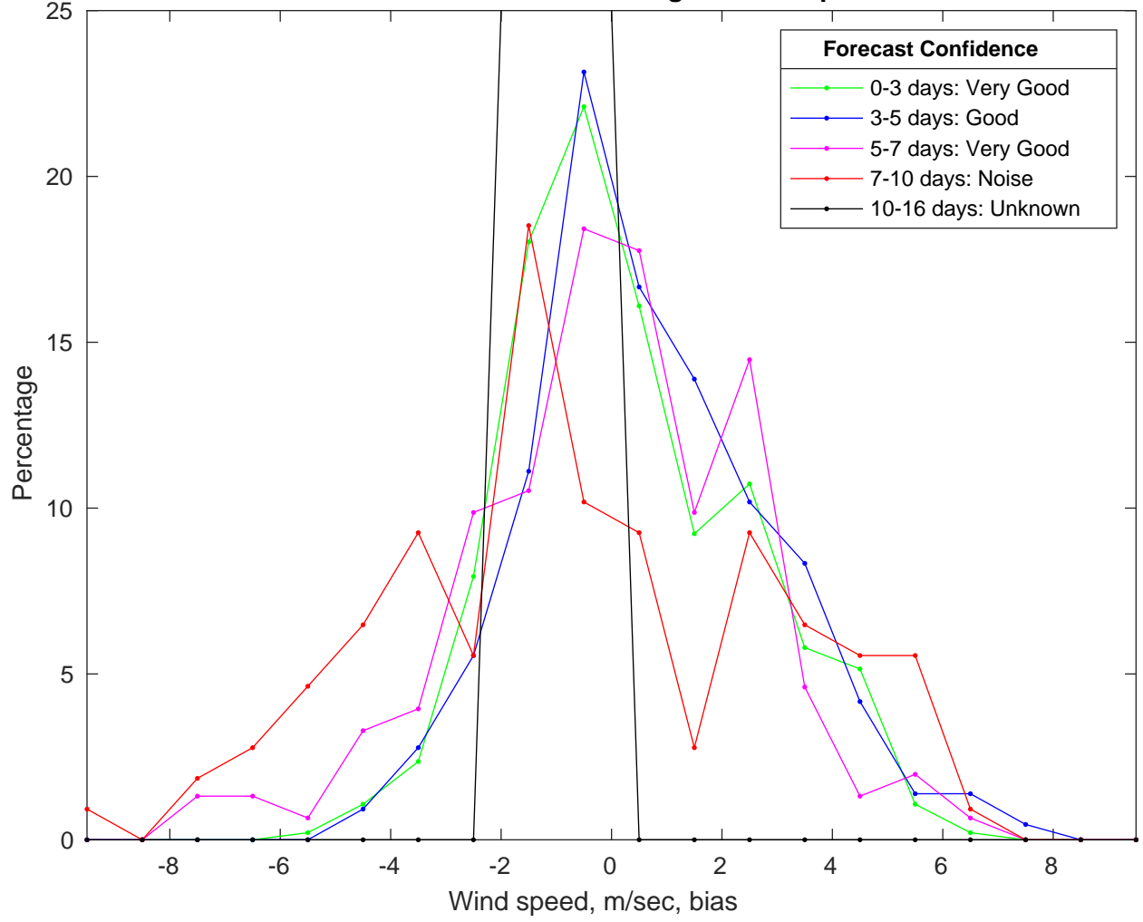
NDBC 46011 vs GFS Winds Bias Histogram: 19-Sep-2024
