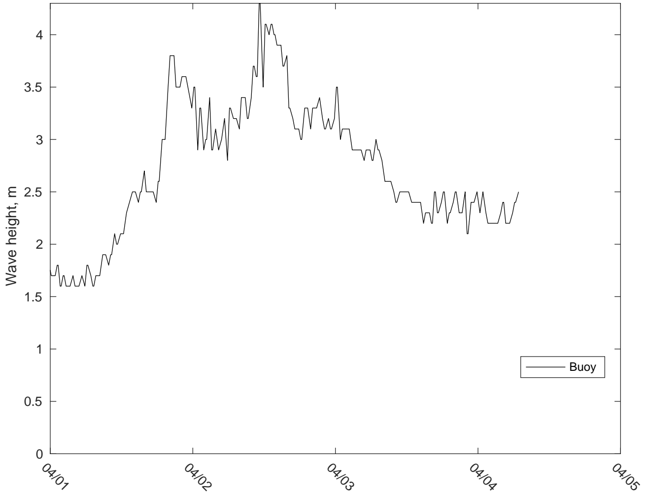
NDBC 46028 vs AUSWAV Waves: 10 to 16 day forecast
