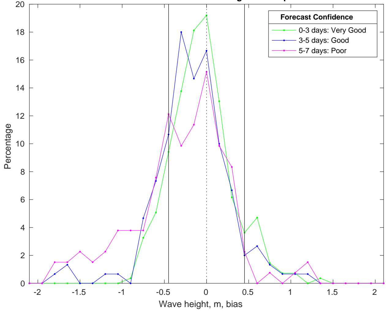
NDBC 46028 vs AUSWAV Waves Bias Histogram: 04-Apr-2025
