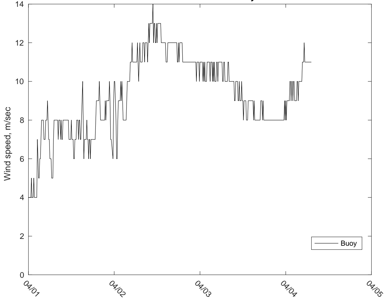
NDBC 46028 vs AUSWAV Winds: 10 to 16 day forecast
