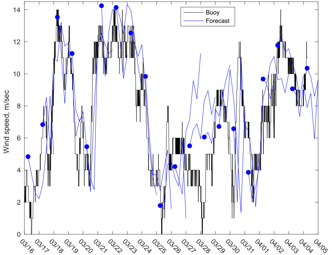
NDBC 46028 vs AUSWAV Winds: 3 to 5 day forecast
