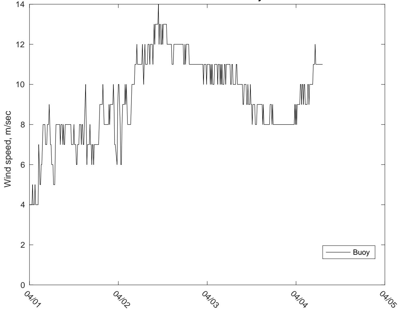
NDBC 46028 vs AUSWAV Winds: 7 to 10 day forecast
