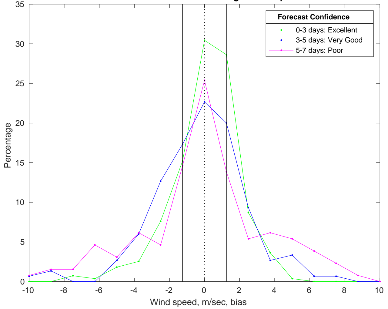
NDBC 46028 vs AUSWAV Winds Bias Histogram: 04-Apr-2025
