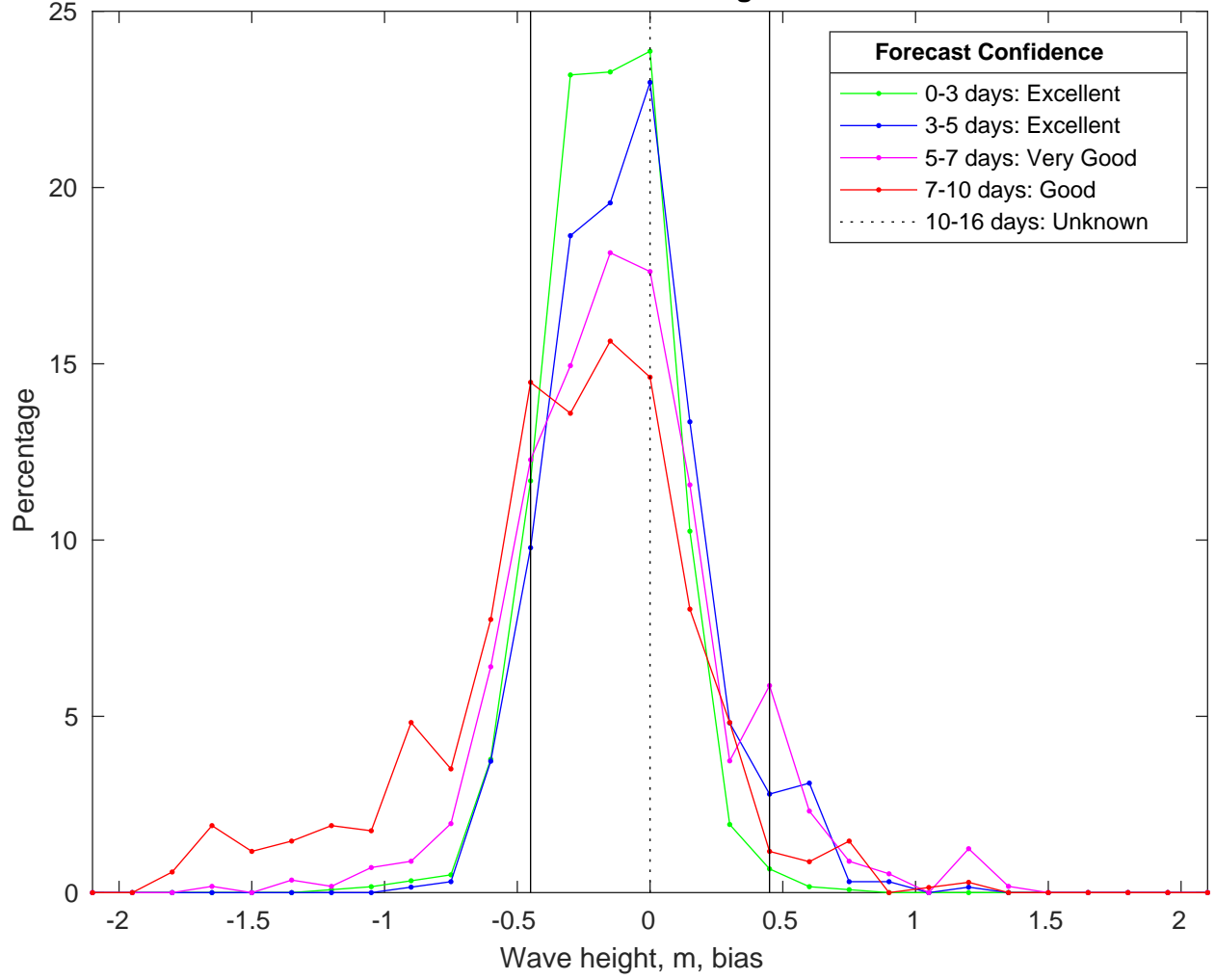
NDBC 46028 vs CMEMSWaves Bias Histogram: 18-Jan-2025
