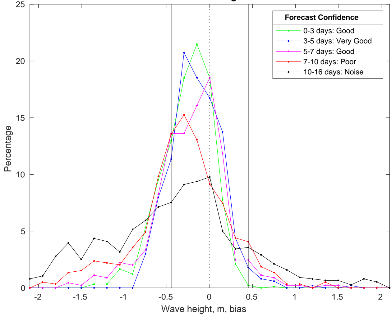
NDBC 46028 vs GFSWaves Bias Histogram: 18-Jan-2025
