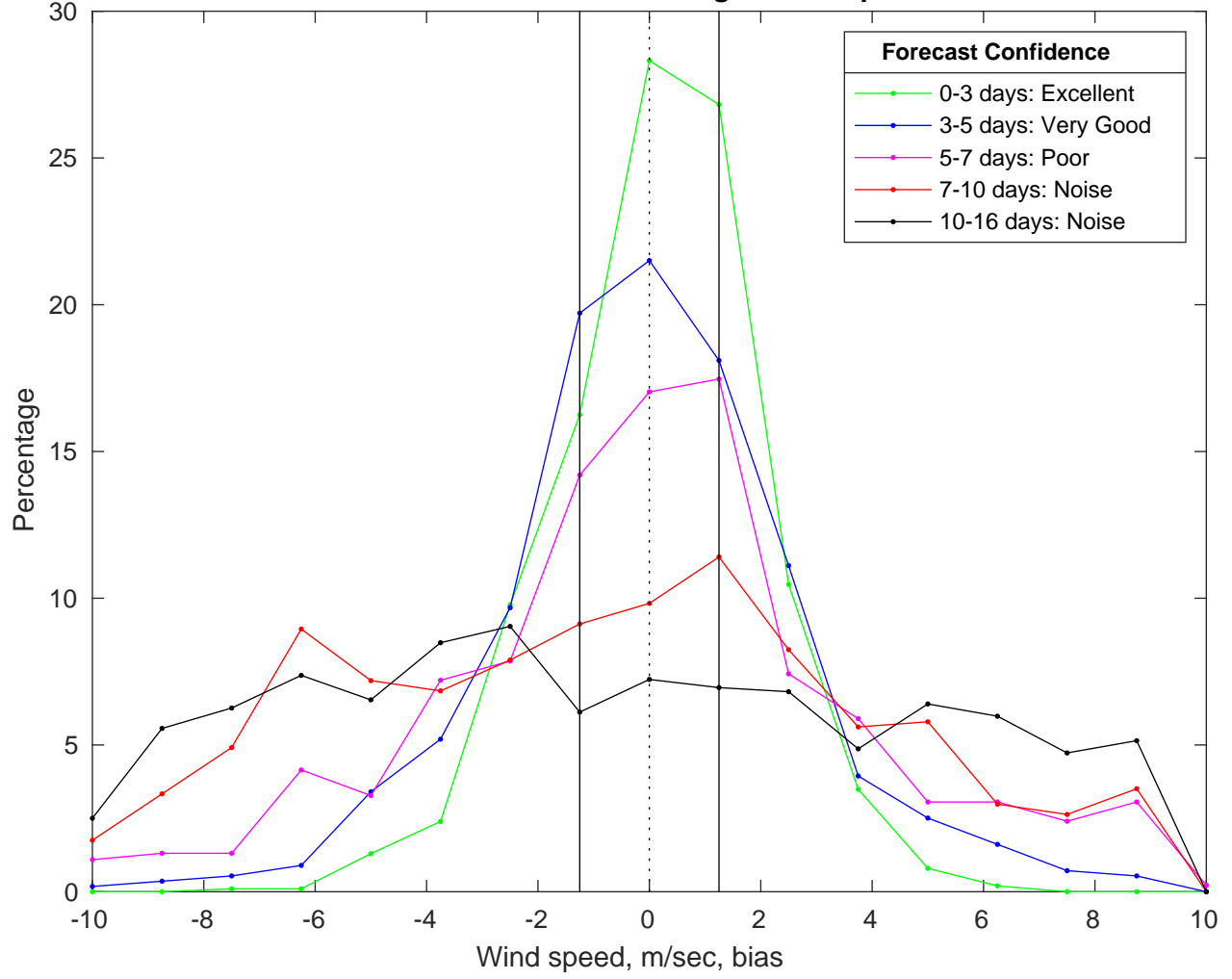
NDBC 46028 vs GFS Winds Bias Histogram: 04-Apr-2025
