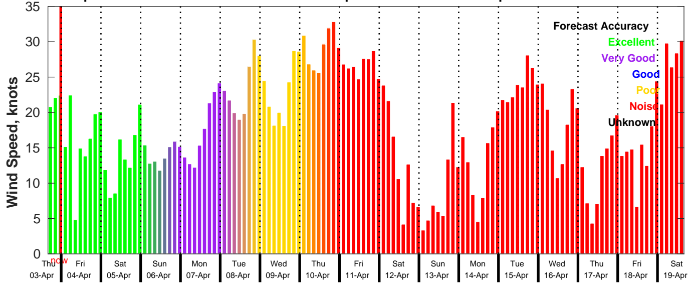
GFS Wind Speed Forecast for NDBC 46028 from 03-Apr-2025 16:00:00 to 19-Apr-2025 16:00:00
