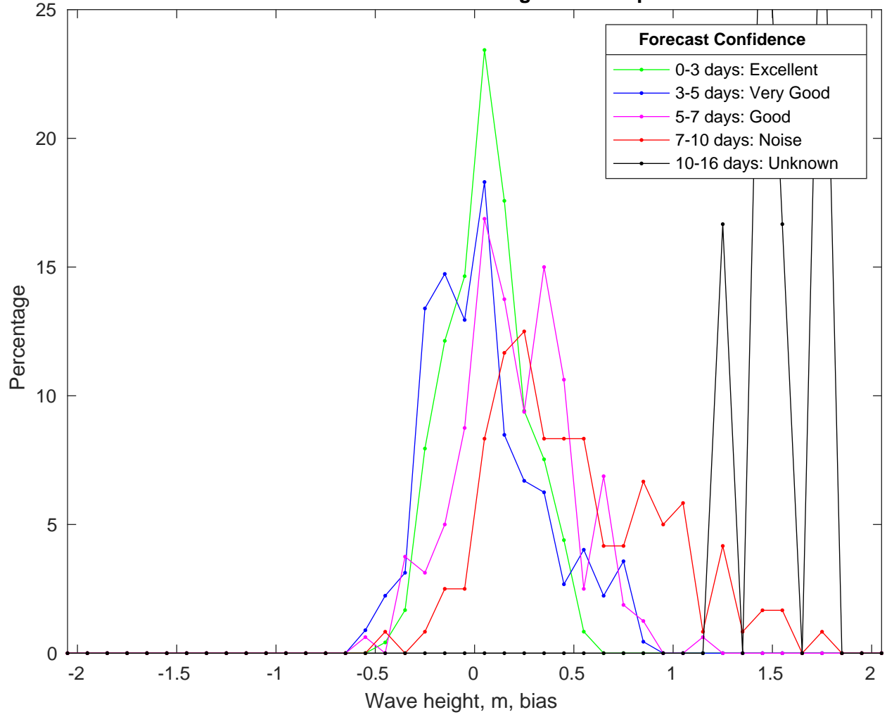
NDBC 46028 vs GFSWaves Bias Histogram: 19-Sep-2024
