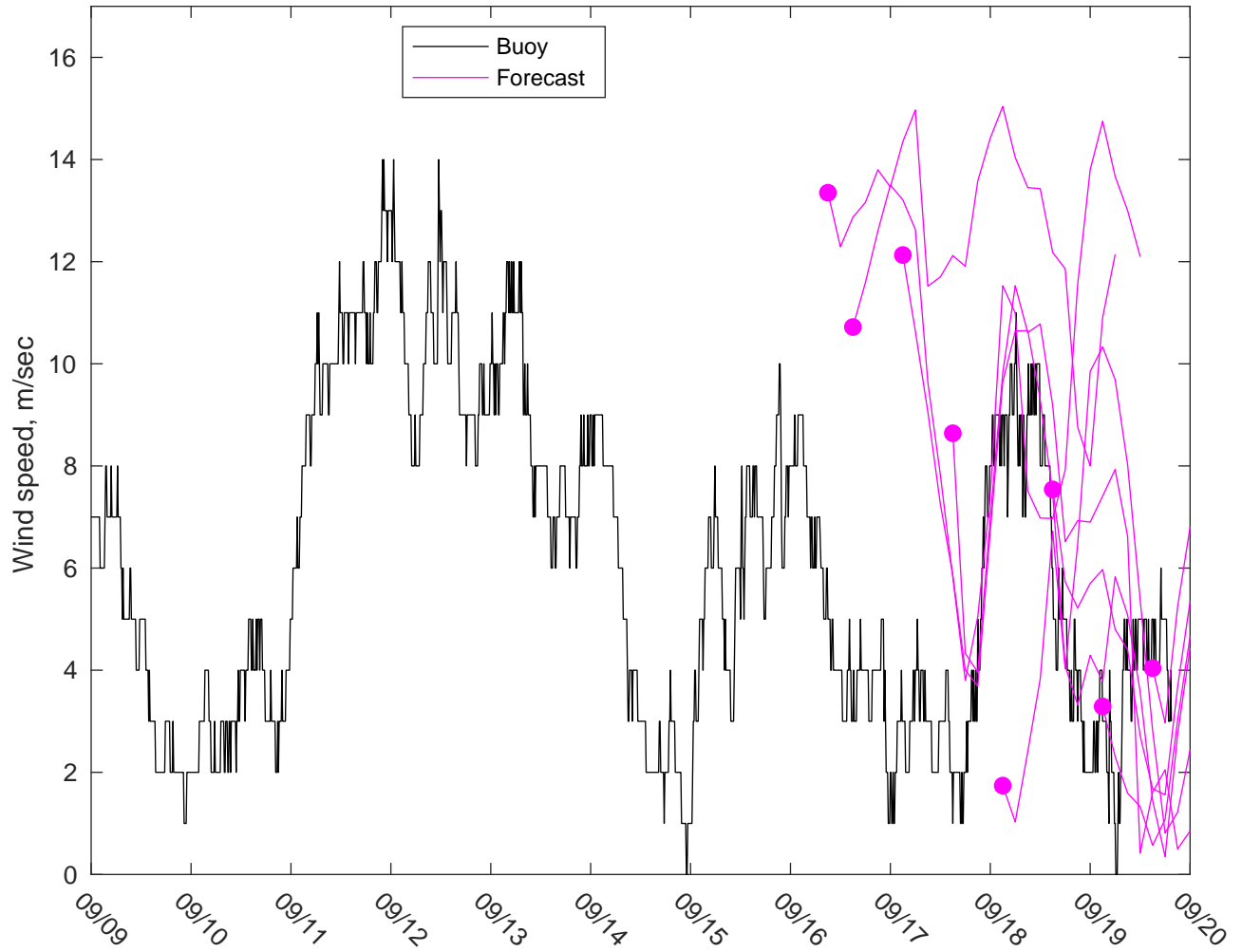
NDBC 46028 vs GFSWinds: 7 to 10 day forecast
