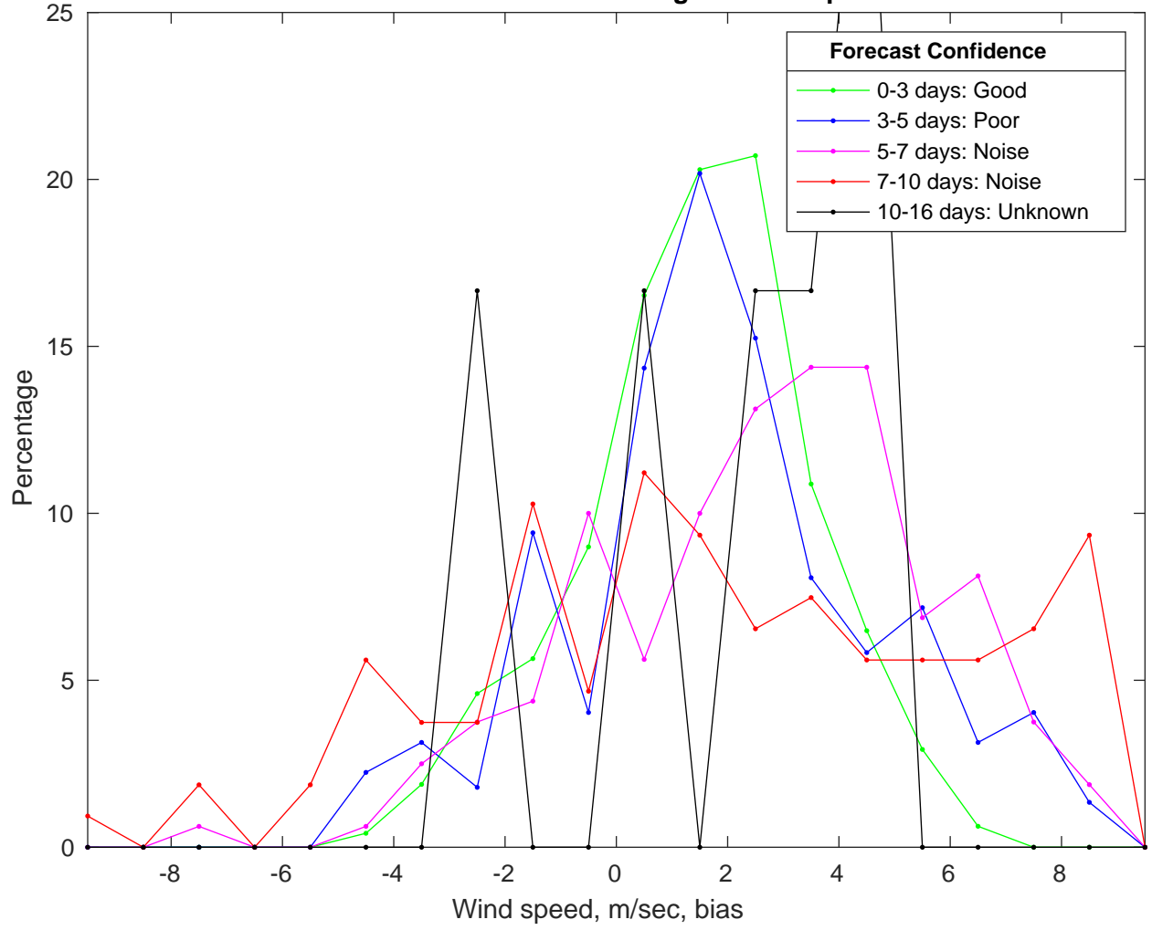
NDBC 46028 vs GFSWinds Bias Histogram: 19-Sep-2024
