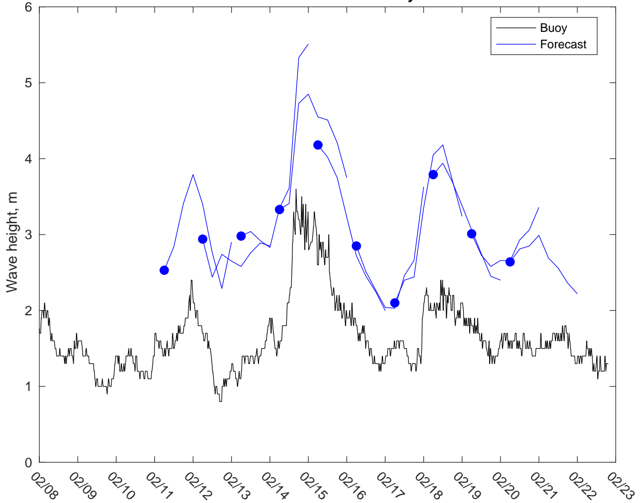
NDBC 46053 vs AUSWAV Waves: 3 to 5 day forecast
