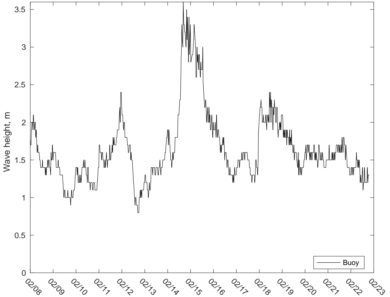
NDBC 46053 vs AUSWAV Waves: 7 to 10 day forecast
