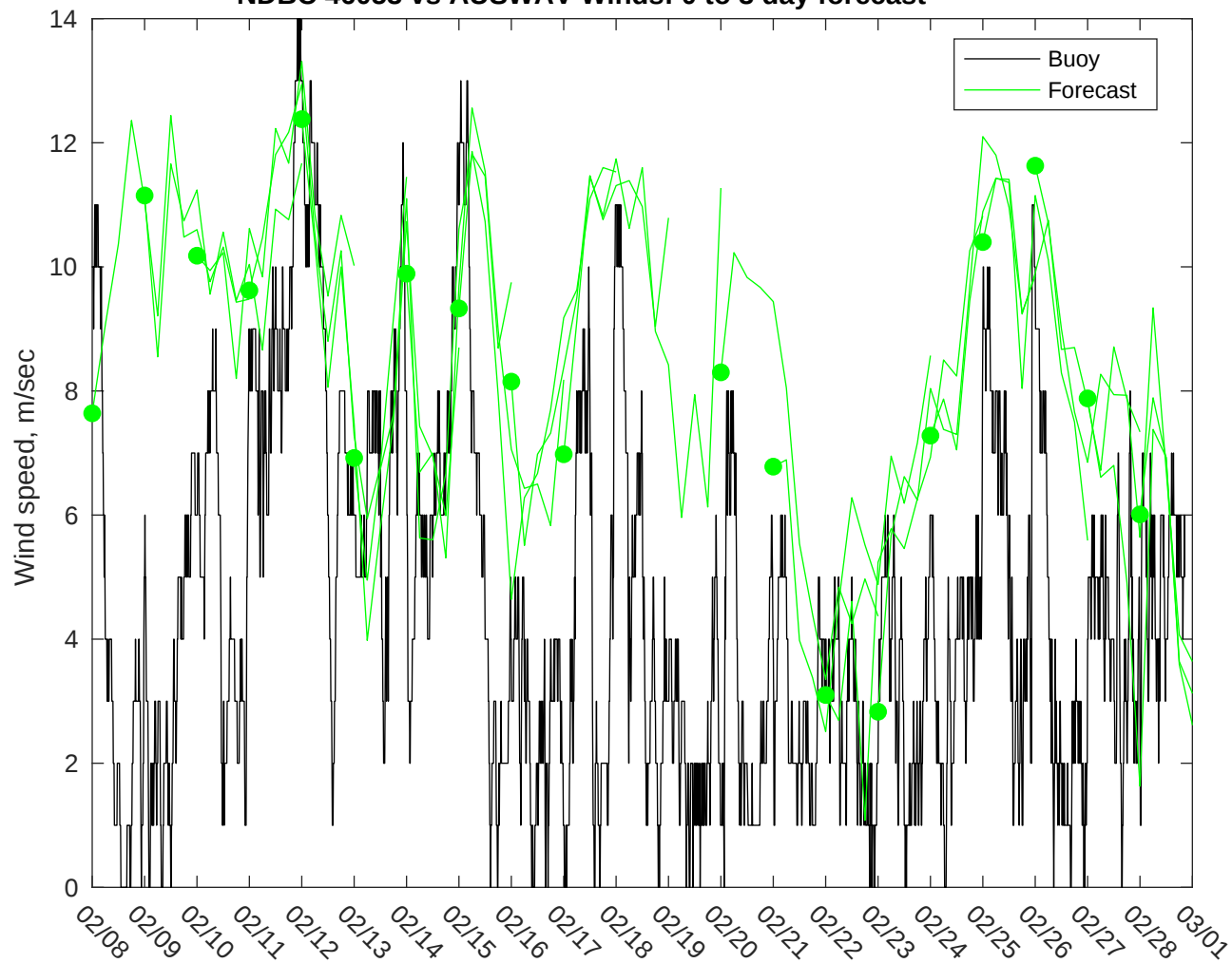
NDBC 46053 vs AUSWAV Winds: 0 to 3 day forecast
