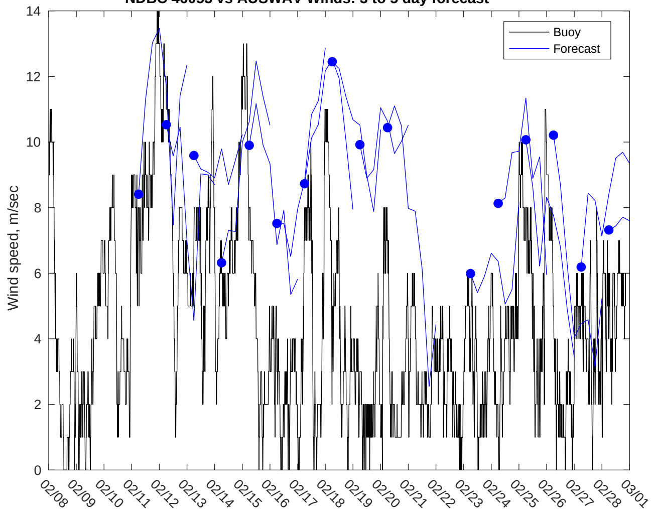
NDBC 46053 vs AUSWAV Winds: 3 to 5 day forecast
