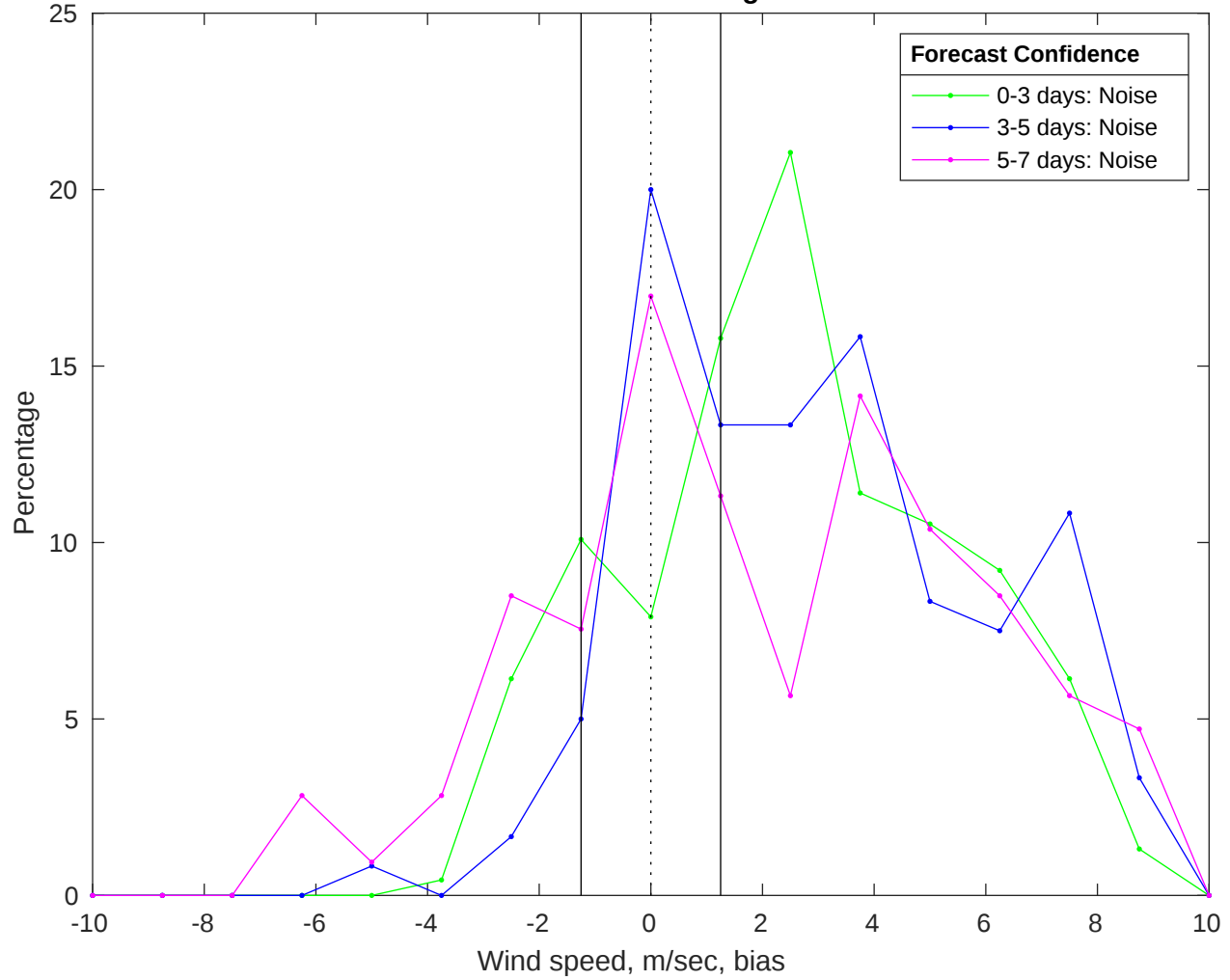
NDBC 46053 vs AUSWAV Winds Bias Histogram: 28-Feb-2025
