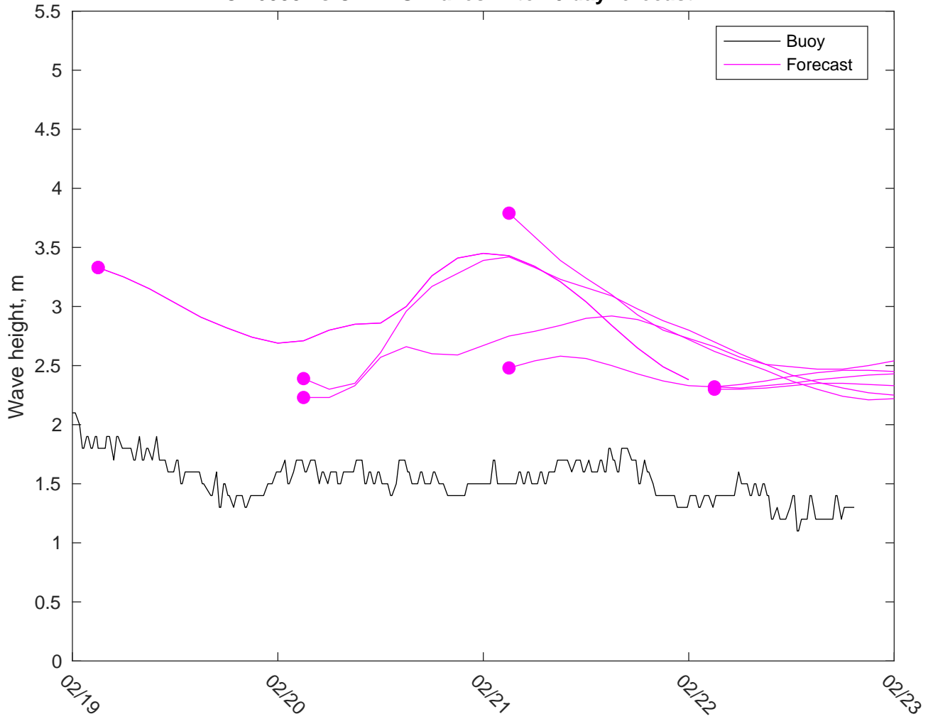
NDBC 46053 vs CMEMS Waves: 7 to 10 day forecast
