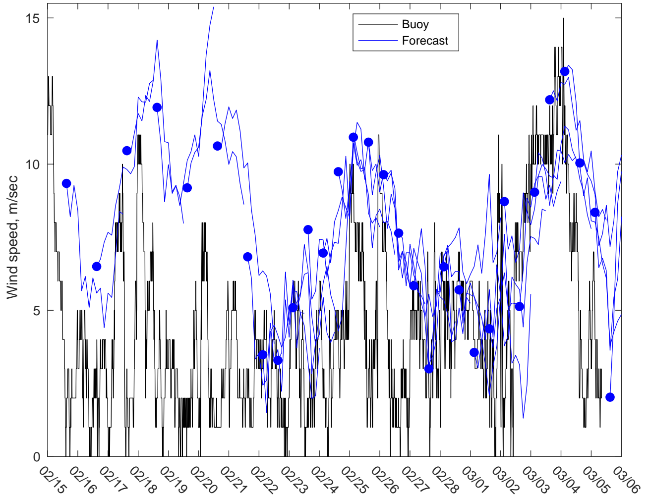
NDBC 46053 vs GFS Winds: 3 to 5 day forecast
