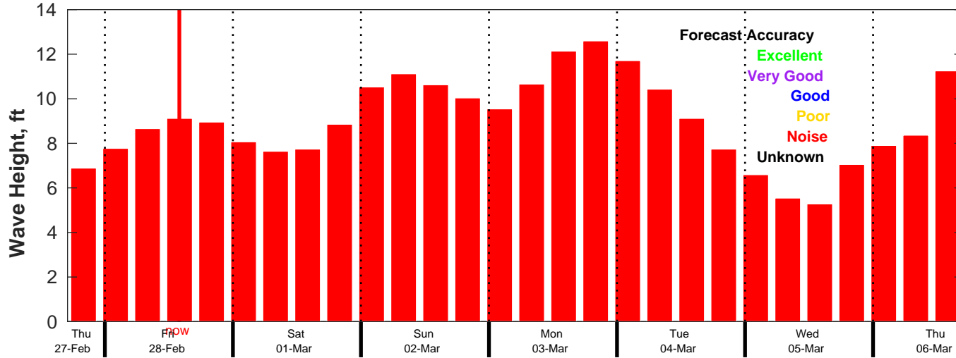
AUSWAV Wave Forecast for NDBC 46053 from 27-Feb-2025 17:00:00 to 06-Mar-2025 17:00:00
