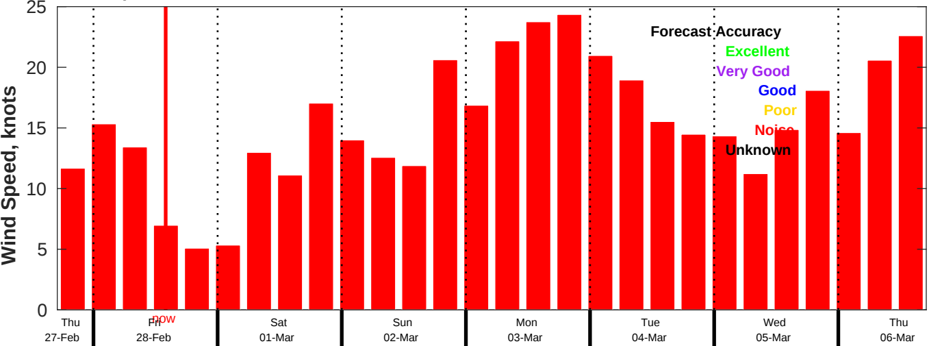
AUSWAV Wind Speed Forecast for NDBC 46053 from 27-Feb-2025 17:00:00 to 06-Mar-2025 17:00:00
