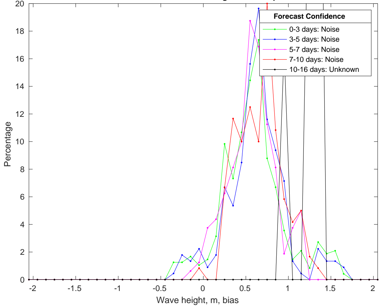
NDBC 46053 vs GFSWaves Bias Histogram: 19-Sep-2024
