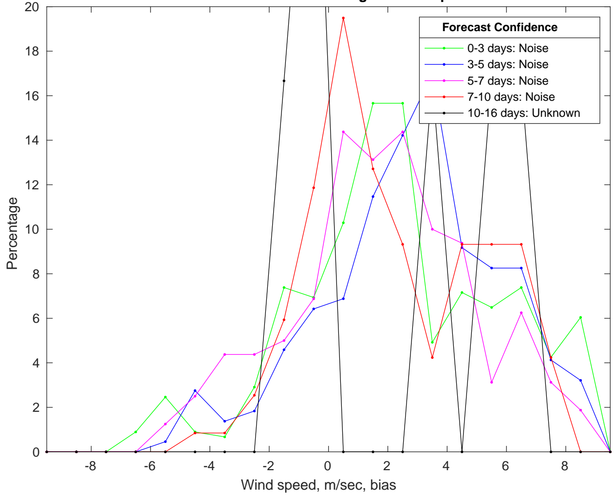
NDBC 46053 vs GFS Winds Bias Histogram: 19-Sep-2024
