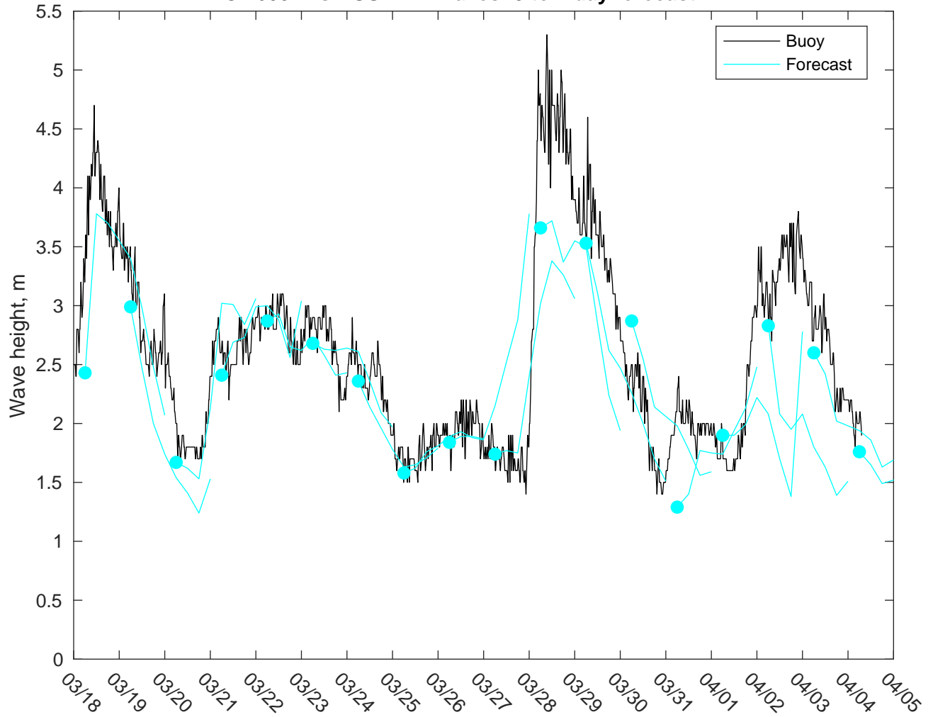
NDBC 46054 vs AUSWAV Waves: 5 to 7 day forecast
