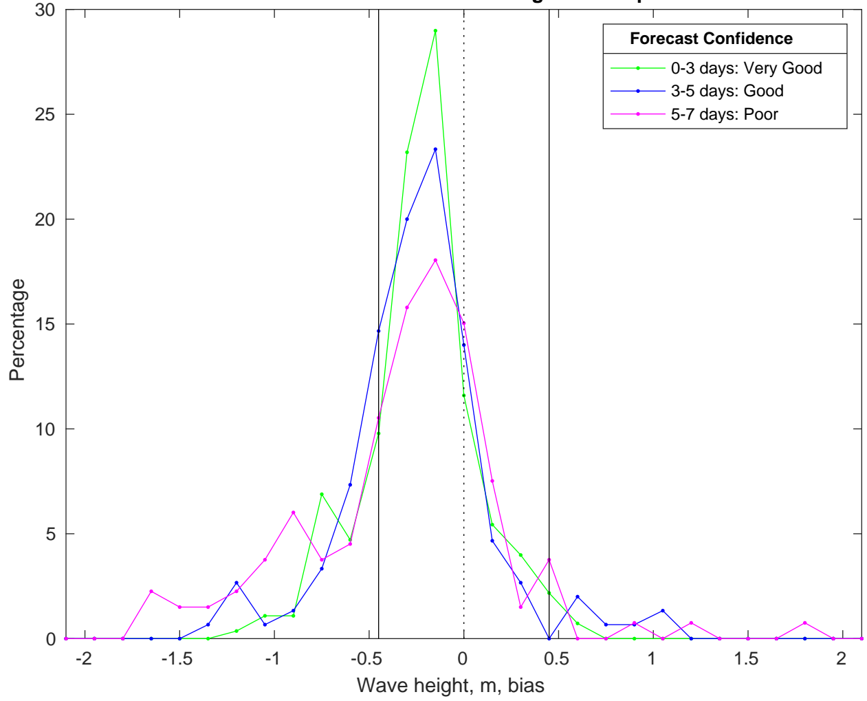
NDBC 46054 vs AUSWAV Waves Bias Histogram: 04-Apr-2025
