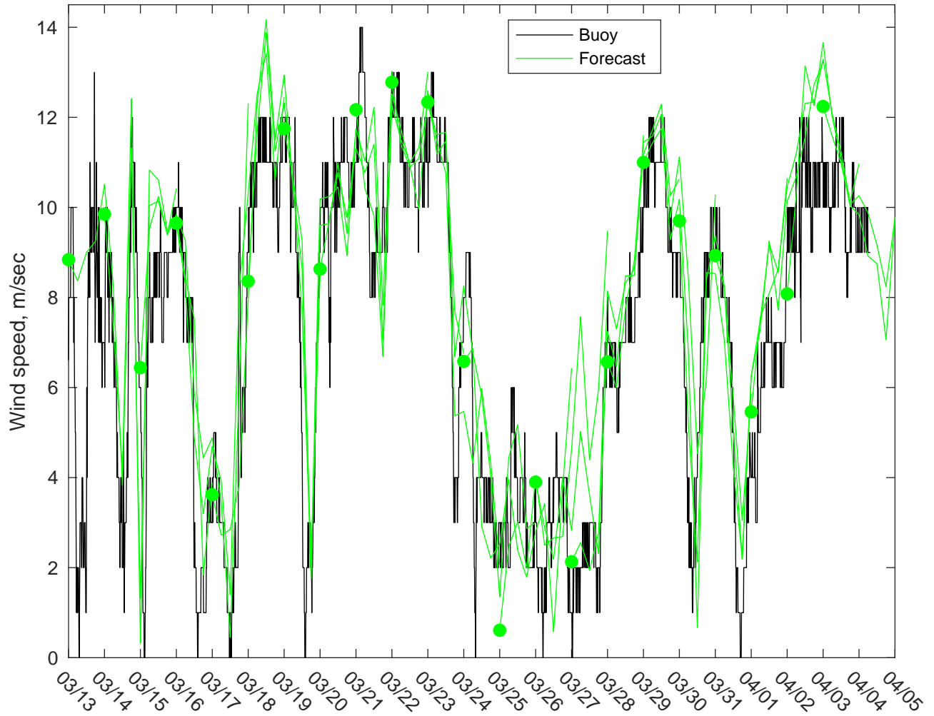
NDBC 46054 vs AUSWAV Winds: 0 to 3 day forecast
