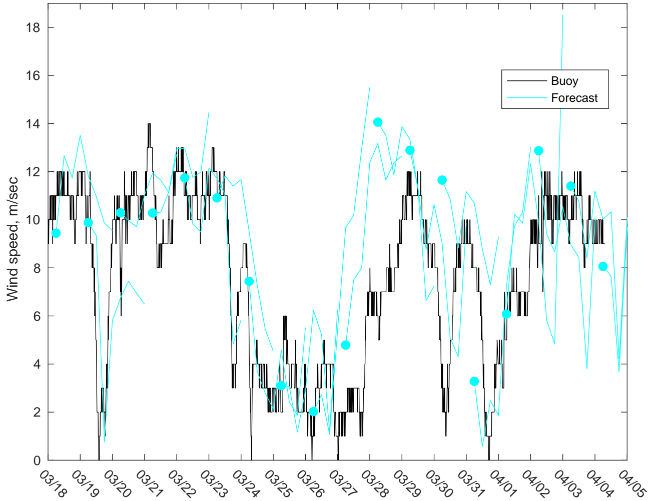
NDBC 46054 vs AUSWAV Winds: 5 to 7 day forecast
