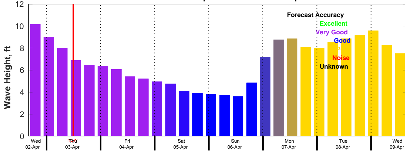
AUSWAV Wave Forecast for NDBC 46054 from 02-Apr-2025 16:00:00 to 09-Apr-2025 16:00:00
