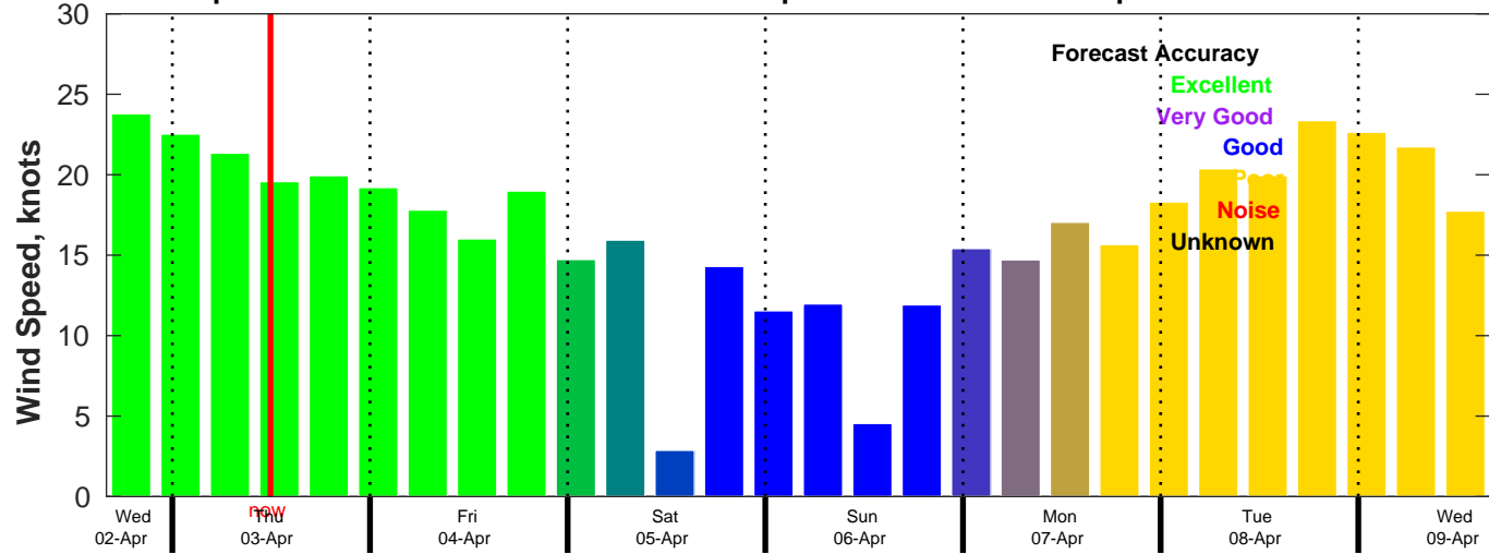
AUSWAV Wind Speed Forecast for NDBC 46054 from 02-Apr-2025 16:00:00 to 09-Apr-2025 16:00:00
