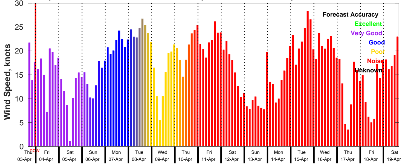
GFS Wind Speed Forecast for NDBC 46054 from 03-Apr-2025 16:00:00 to 19-Apr-2025 16:00:00
