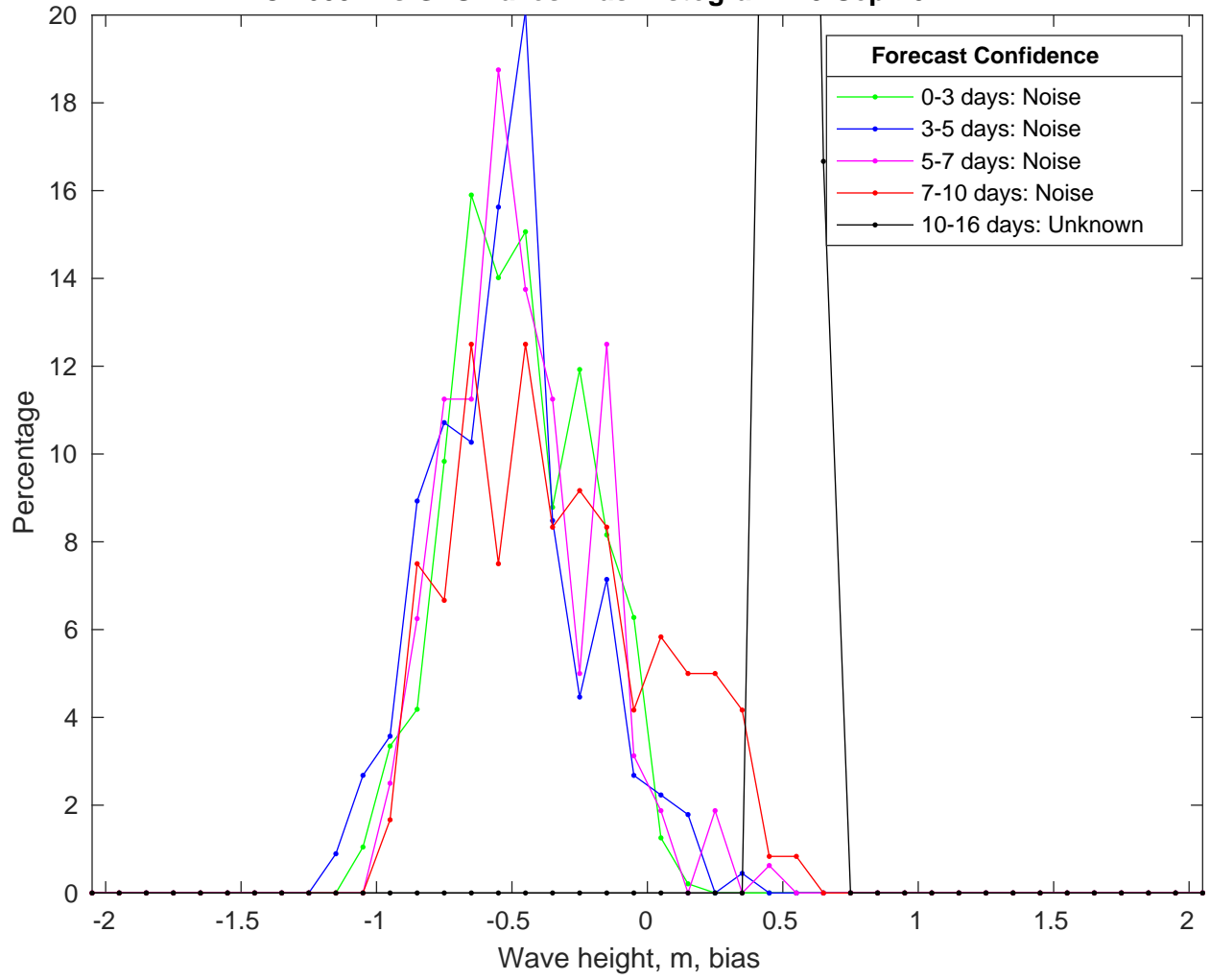
NDBC 46054 vs GFSWaves Bias Histogram: 19-Sep-2024
