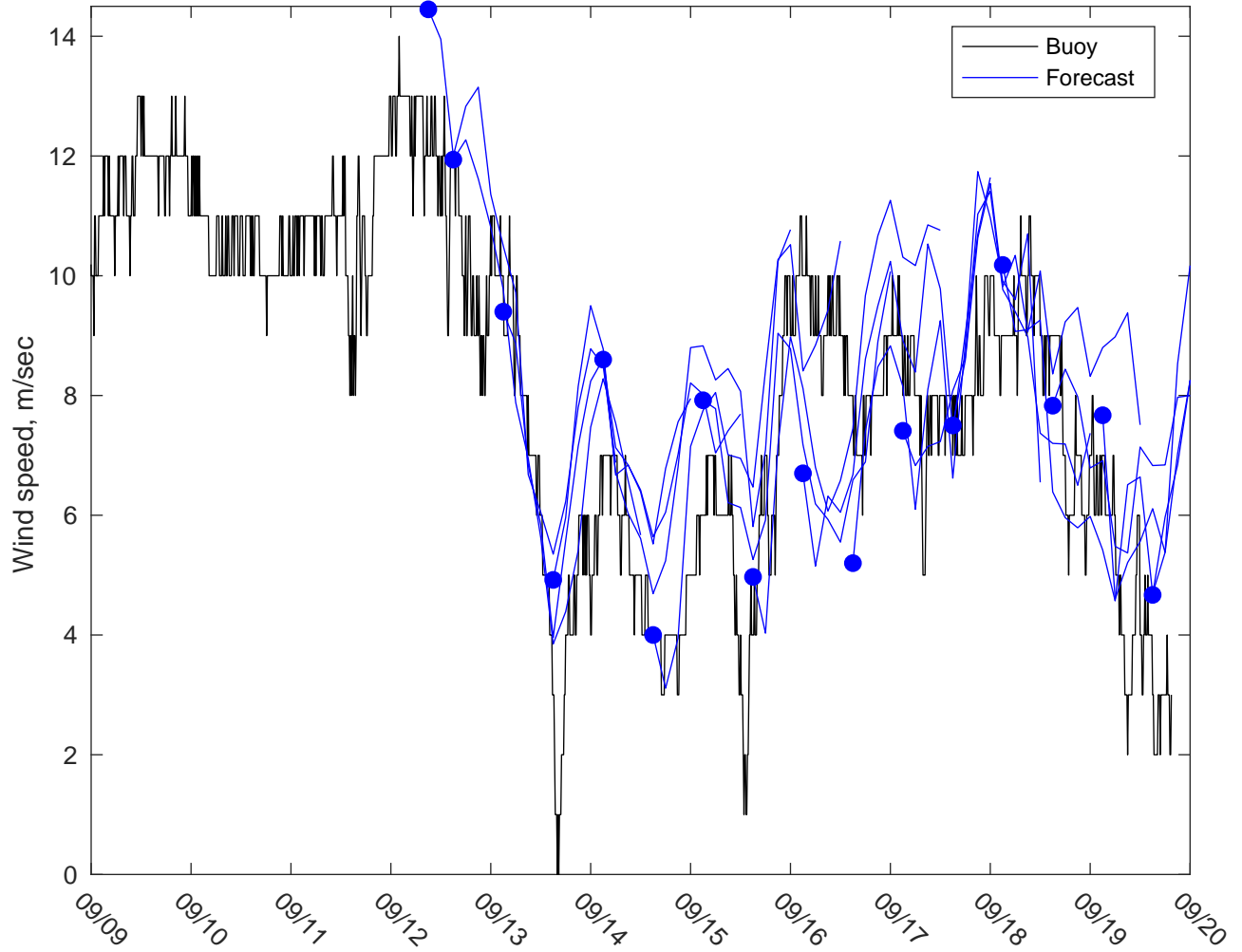
NDBC 46054 vs GFSWinds: 3 to 5 day forecast
